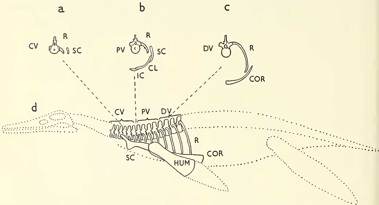
TEXT-FIG. 3. Diagram showing probable position of scapula of Stretham Pliosaurus in the body. a , transverse section through posterior part of neck and dorsal process of scapula. b , transverse section through anterior part of thorax and clavicular arch. c , transverse section through posterior part of thorax and coracoid. d , lateral view of thorax and pectoral girdle. CL., Clavicle; COR., Coracoid; HUM., Humerus; IC., Interclavicle; R., Rib; SC., Scapula; v., Vertebrae (CV., cervical; PV., pectoral; DV., dorsal).
